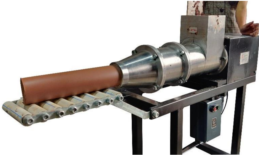
Pug Mill
